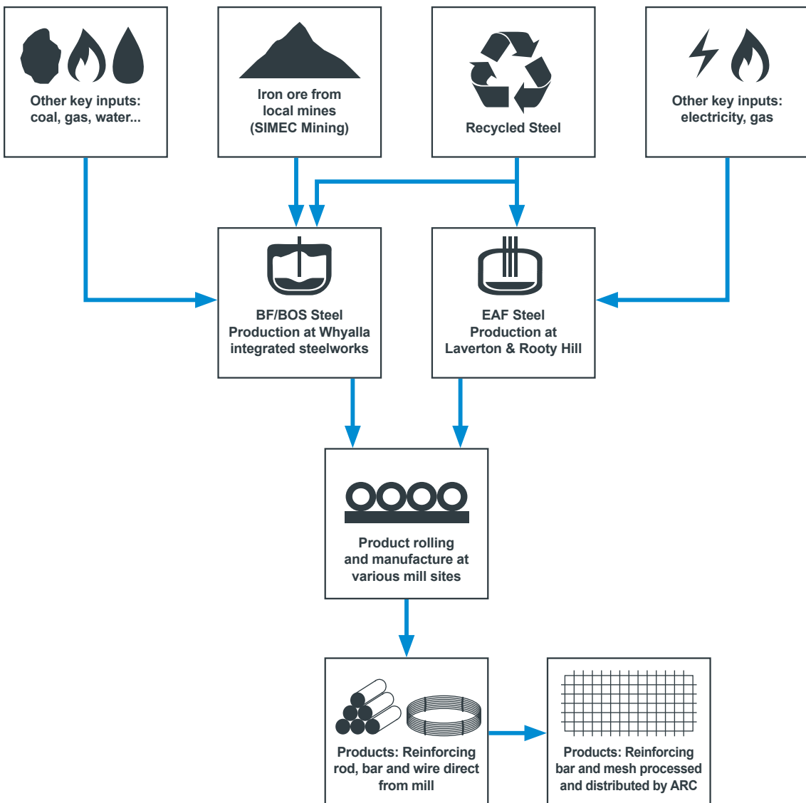
Figure 3: Reinforcing bar and mesh products manufactured by ARC
