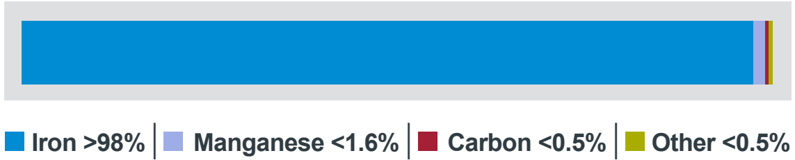
Figure 2: The typical composition of ARC's reinforcing bar and mesh
